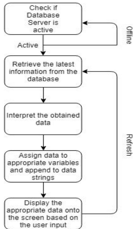
Fig 4: Software Flow Diagram
