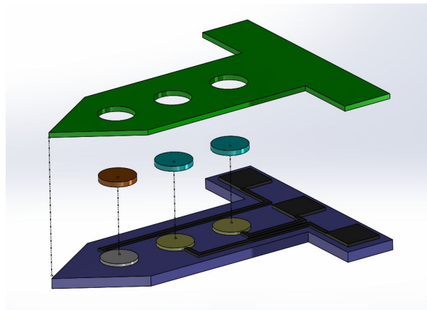
Fig 2: A diagram showing the components of the sensor.
