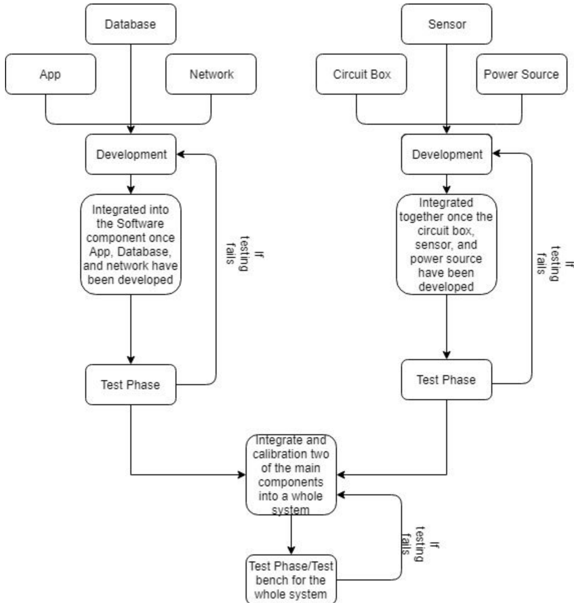
Fig 8: Process Flowchart
